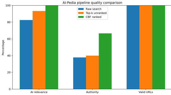
Fig. 10. Comparison of raw search, unranked top- K , and CBF-ranked top- K outputs. Ranking improves both AI relevance and source authority, and the main compression effect comes from reducing the candidate pool from 201 resources to 15.
